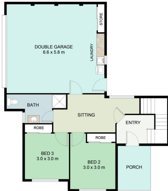
LOWER FLOOR PLAN
